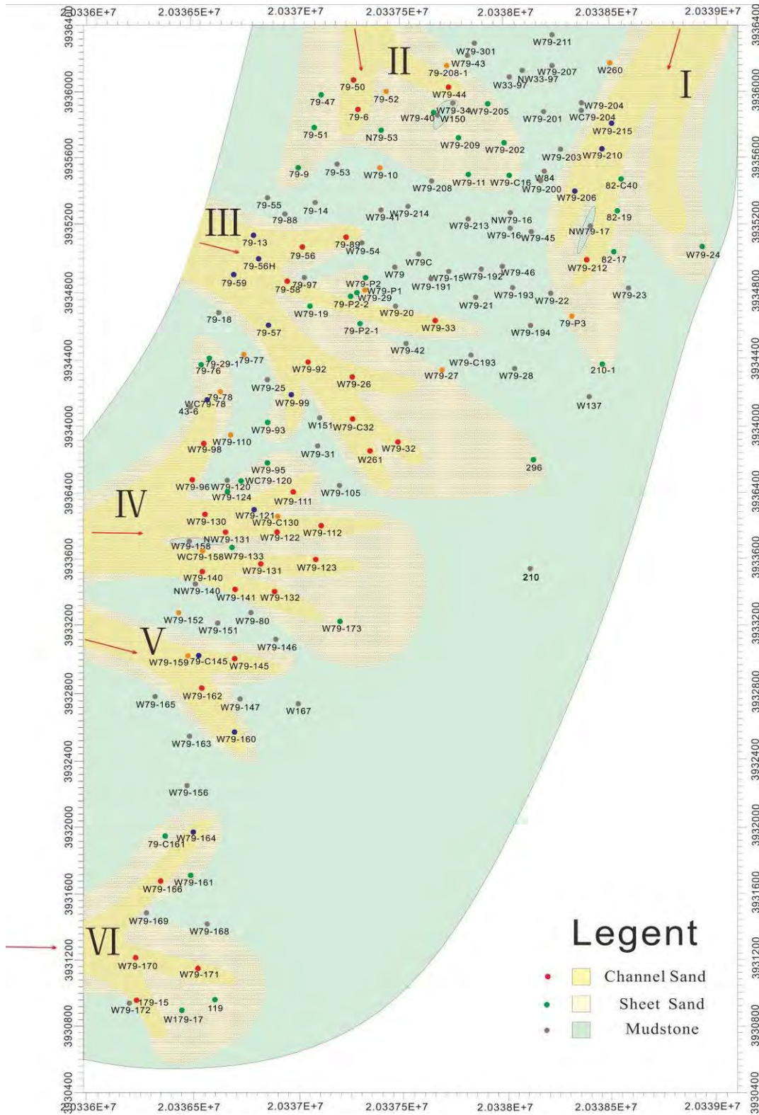
Figure 5. S2L4 10 single underwater distributary channel plane distribution map
