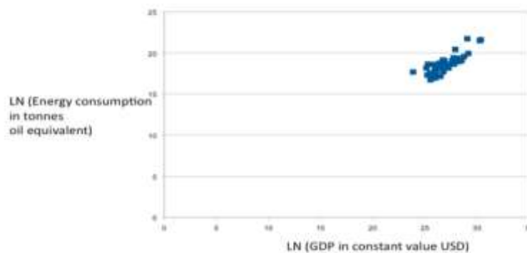
Diagram 4. GDP and energy consumption: \text{LN GDP} - \text{LN energy consumption}: y=0.71x, R^2=0.695 .
